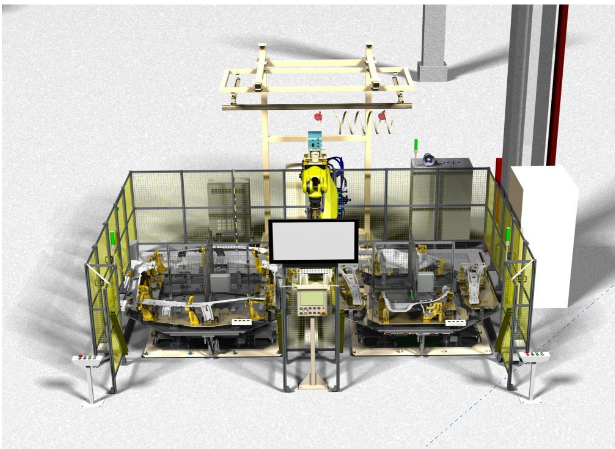
沖壓自動搬送線 Automatic handling line for stamping
