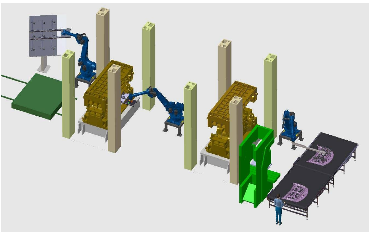
沖壓自動搬送線 Automatic handling line for stamping
