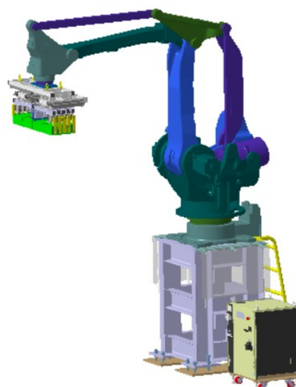
機械手磚塊堆疊設備 Robotic stacking equipment
